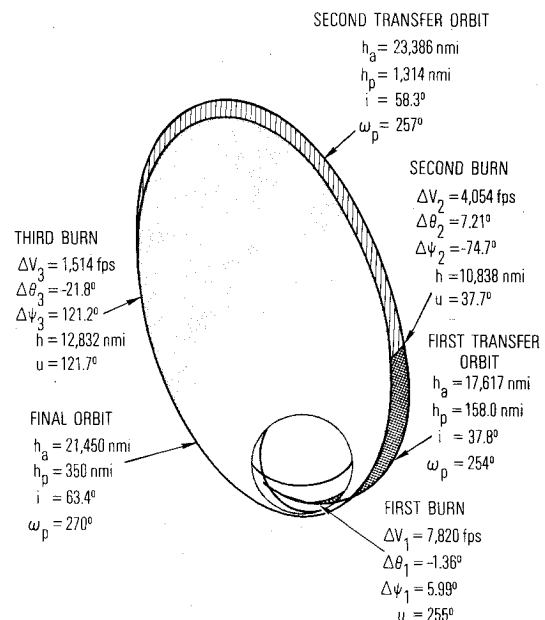
Fig. 2 Optimal three-burn transfer, i = 63.4^\circ .
