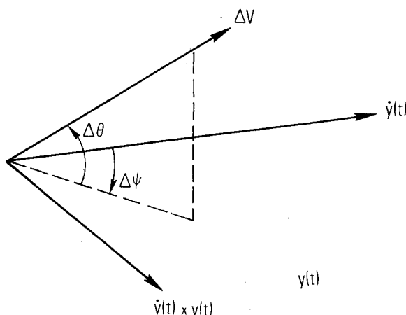
Fig. 1 Definition of yaw increment, \Delta\psi , and pitch increment, \Delta\theta .
