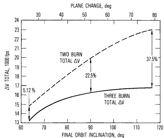
Fig. 4 Impulsive burn incremental velocities.
