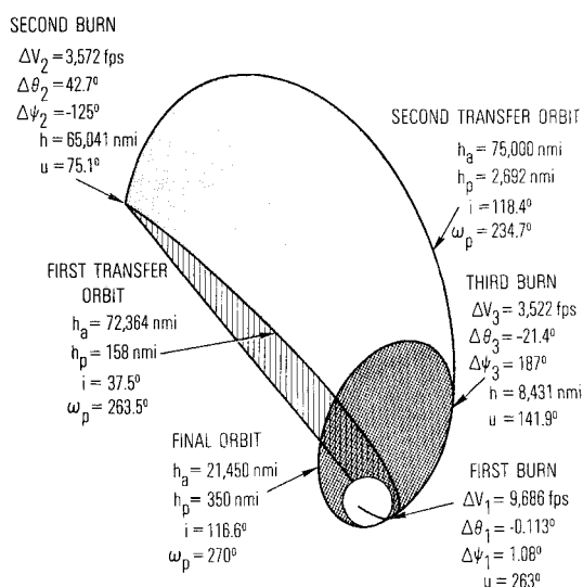
Fig. 3 Optimal three-burn transfer, i = 116.6^\circ .
